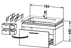
# 6447 ↔ 780 mm, ↗ 490 mm → # 0491800000, 800 mm → # 0491800030, 800 mm
