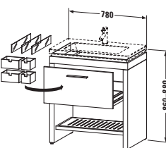
# 6457 ↔ 780 mm, ↗ 490 mm → # 0491800000, 800 mm → # 0491800030, 800 mm
