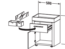
# 9272 ↔ 500 mm, ↗ 360 mm
