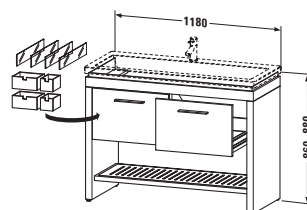
# 6458 ↔ 1180 mm, ↗ 490 mm → # 0491120000, 1200 mm → # 0491120030, 1200 mm → # 0491120024, 1200 mm
