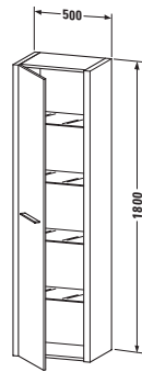
# 9156 L/R ↔ 500 mm, ↗ 360 mm
