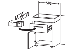
# 9272 ↔ 500 mm, ↗ 360 mm
