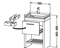
# 6456 ↔ 580 mm, ↗ 420 mm → # 0491600000, 600 mm → # 0491600030, 600 mm
