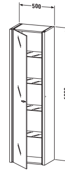
# 9157 L/R \text{⊗} 4 x 21 W ↔ 500 mm, ↗ 360 mm
