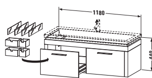
# 6448 ↔ 1180 mm, ↗ 490 mm → # 0491120000, 1200 mm → # 0491120030, 1200 mm → # 0491120024, 1200 mm
