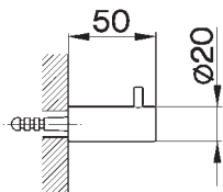
SY 09071 0 Appendino singolo Single hook Crochet single Einzelwandhaken Percha simple
