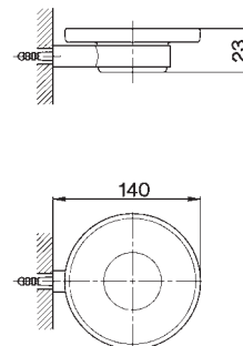
SY 09060 0 Porta sapone Soap holder Porte-savon Seifenhalter Jabonera
