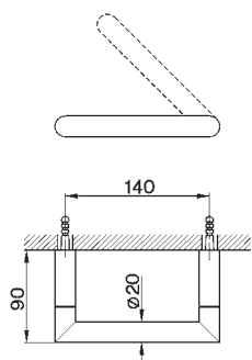
SY 09040 0 Porta rotolo Toilet paper holder Porte-papier Papierrollenhalter Portarrollo
